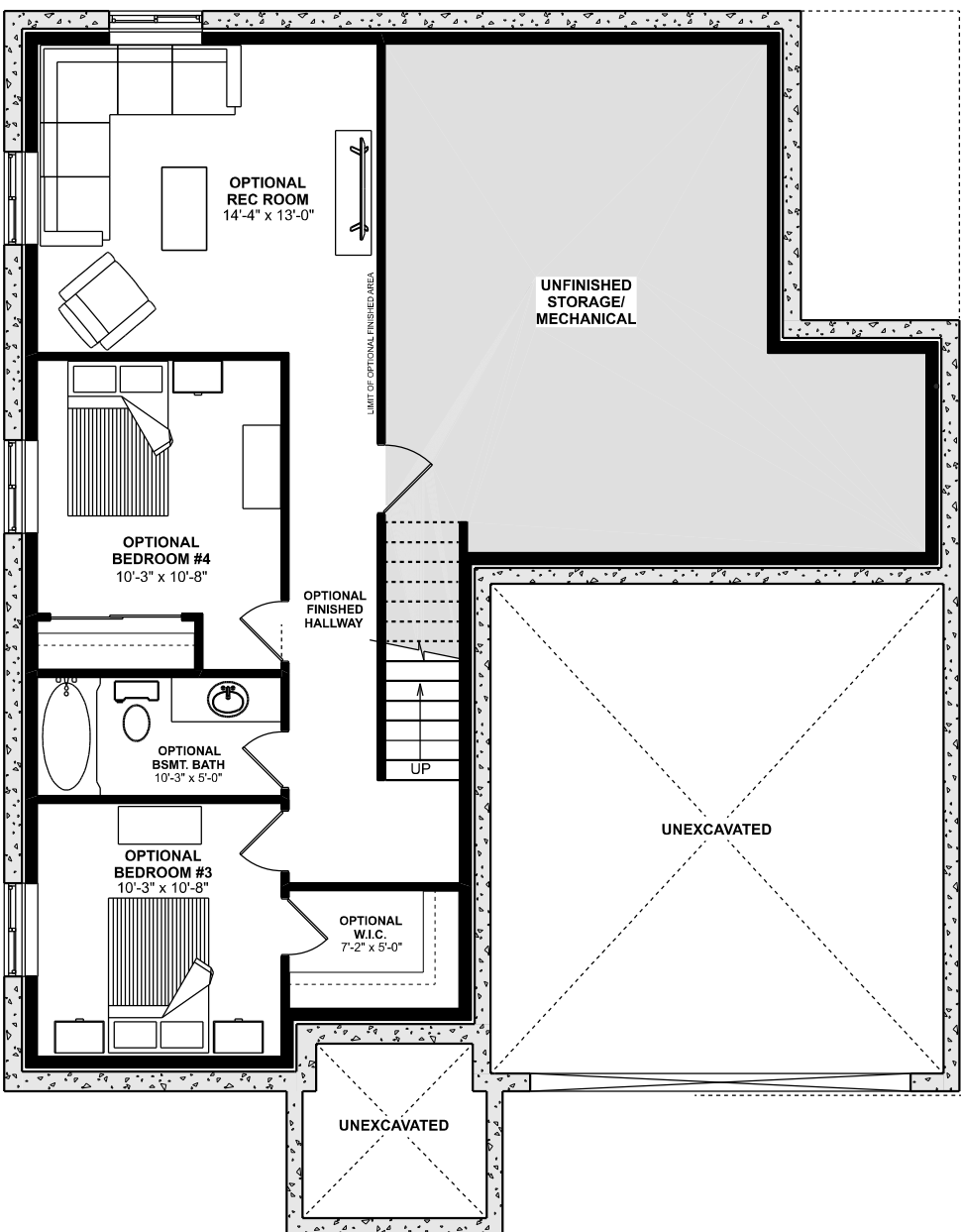
OPTIONAL FINISHED BASEMENT 636 SQFT *INTERIOR OF FRAMED WALLS
